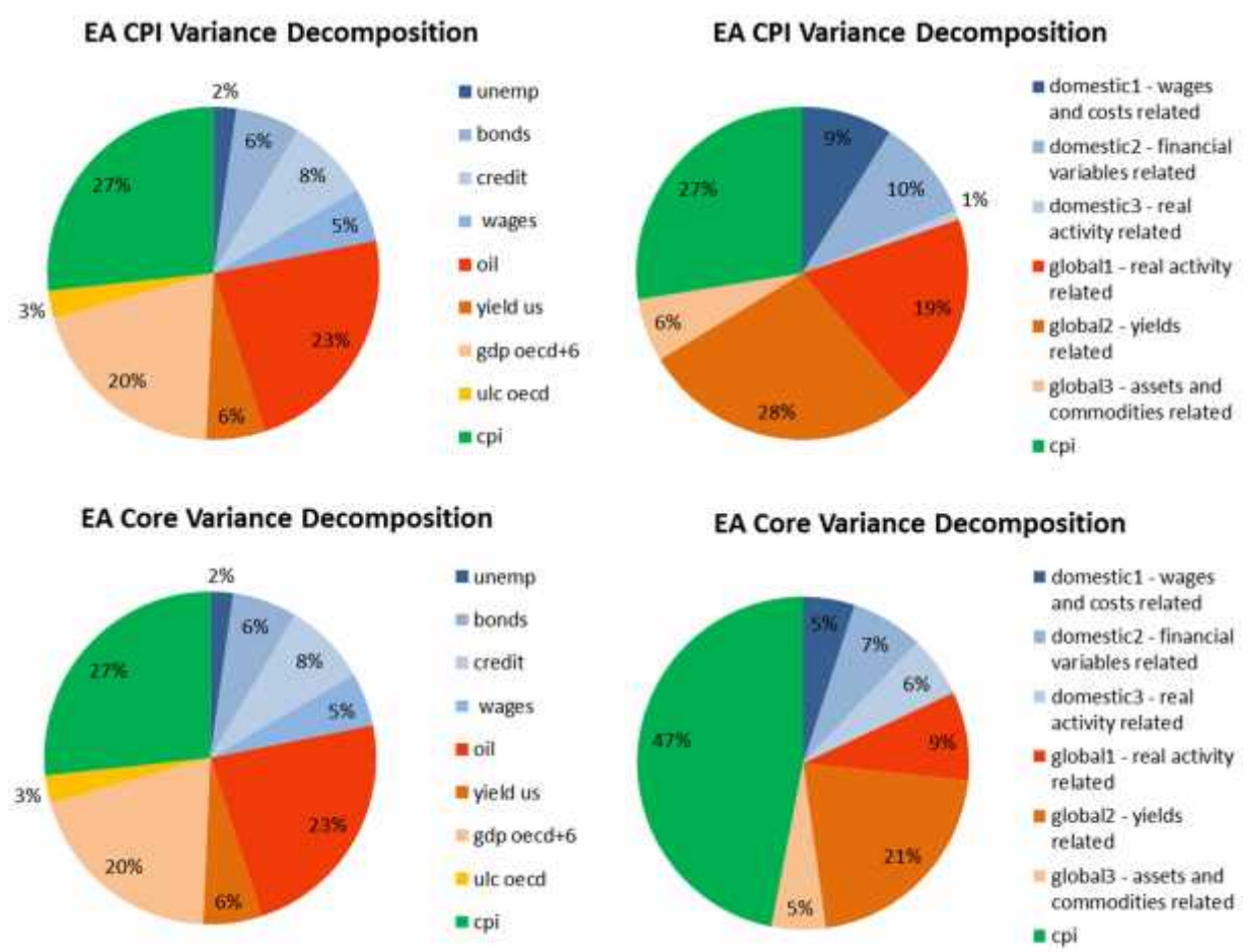
Figure 2 – Variance decomposition
