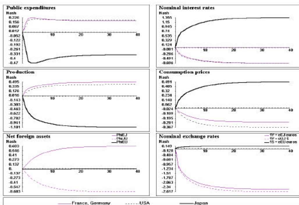
Figure 5: Nash equilibrium with heterogeneous loss functions
