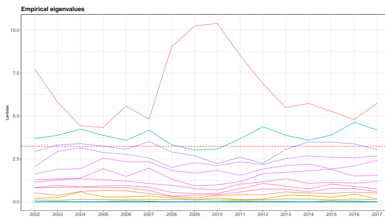
(a) Eigenvalues evolution. Dashed lines represent the upper and lower bounds of the Marchenko-Pastur distribution.
