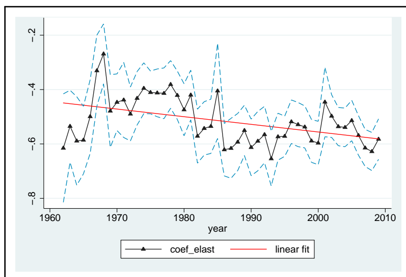
Figure 8: Estimated (1 - \tilde{\sigma})
