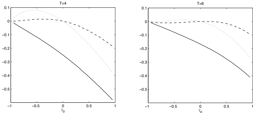
Figure 1. Inconsistencies in the stationary Gaussian autoregression
