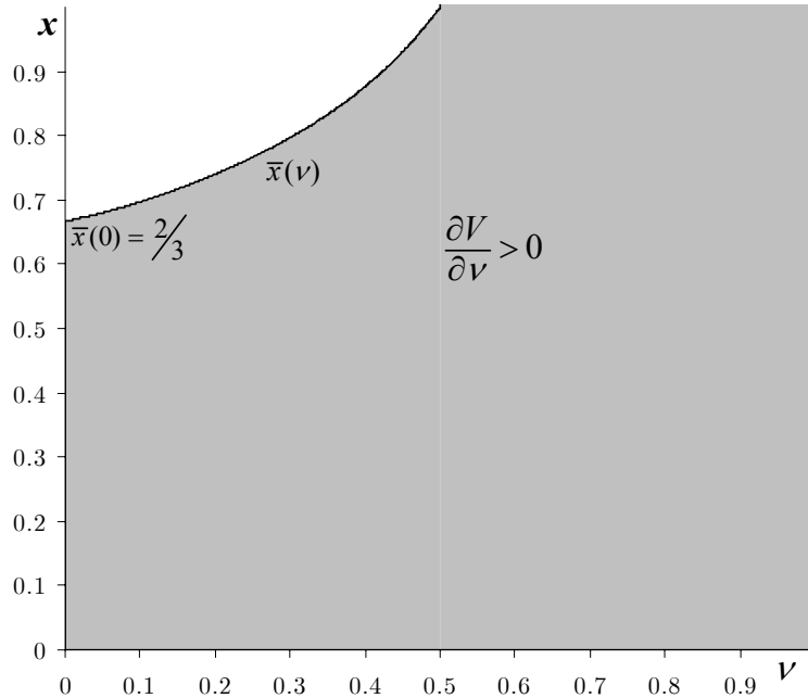
Figure 1: \frac{\partial V}{\partial \nu} as a function of \nu and x .
